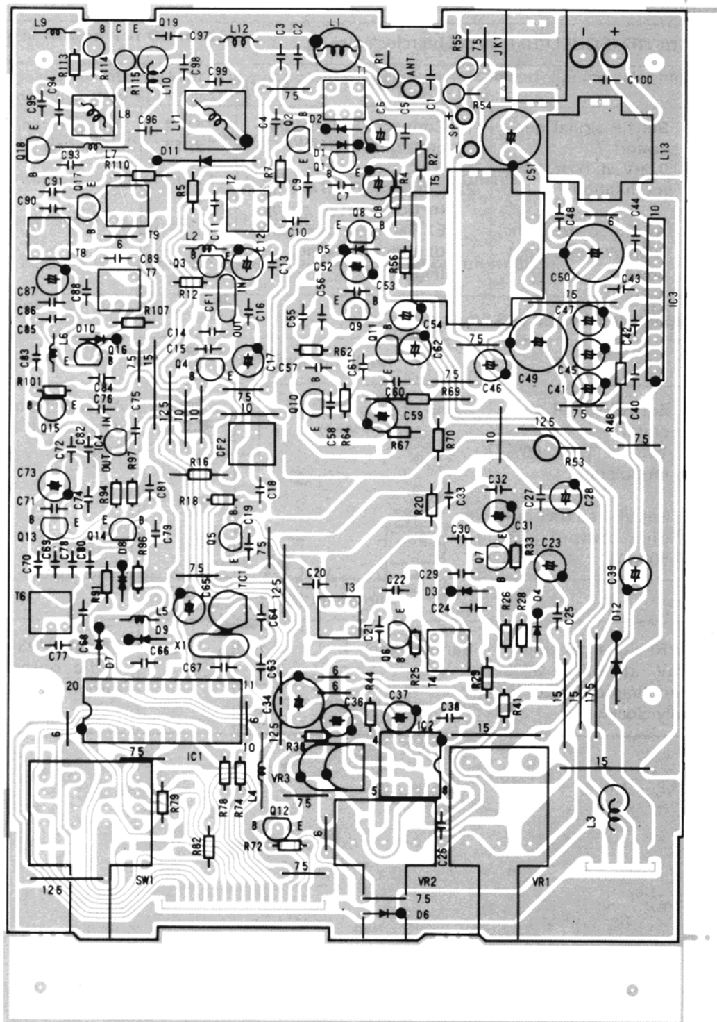
Top View
